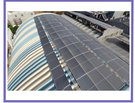
Mounting on Dom Shed
